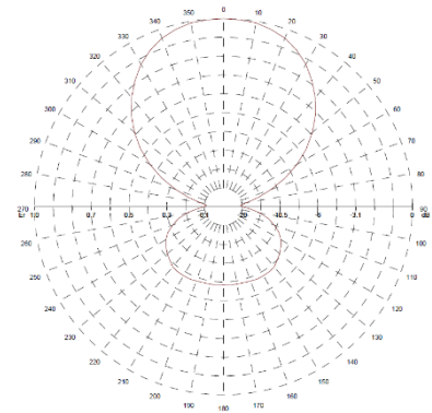
V plane
