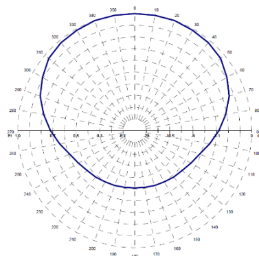
H plane
